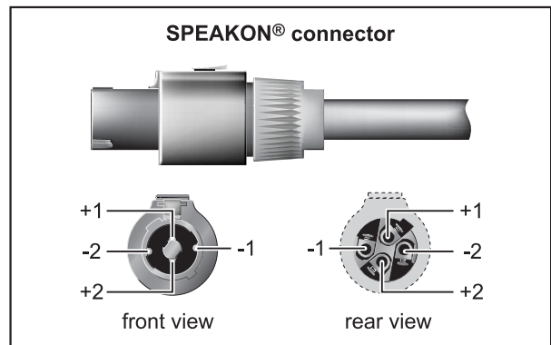
Fig. 4.5: SPEAKON® connector
