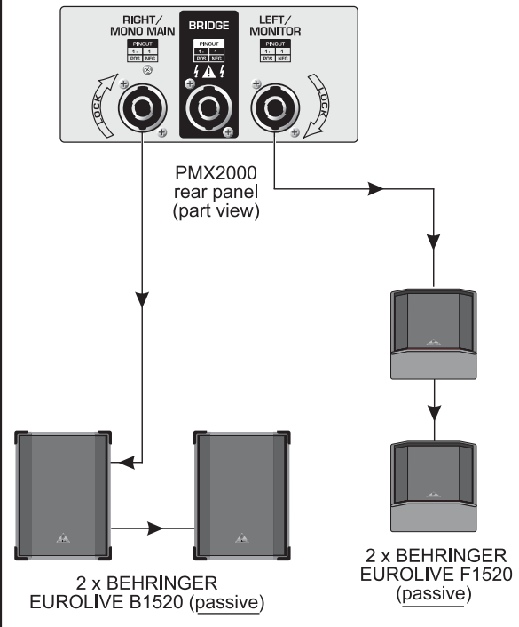
Fig. 5.2: PMX2000 as double mono amplifier (example)
