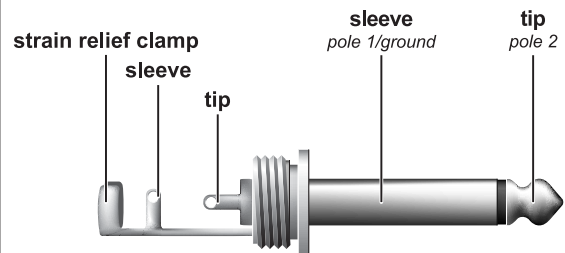
Fig. 4.4: 1/4" TS connector for footswitch
