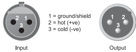
Fig. 4.3: XLR connectors
